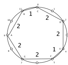
Major heptatonic key of C
