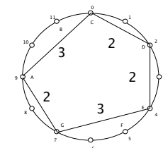
Major pentatonic key of C
